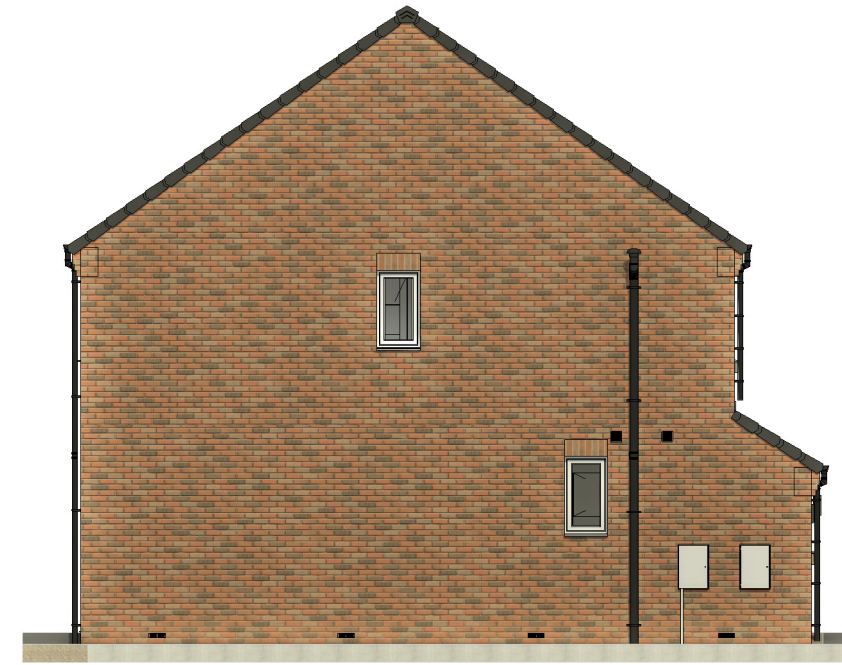
Left Elevation. 1 : 100
